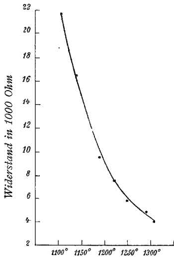
Fig. 6. Quarz III.
